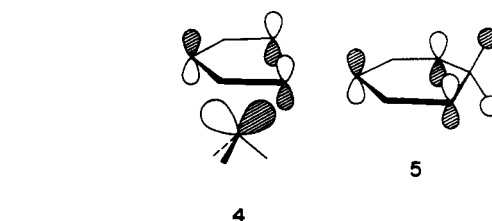
Figure 2. A perturbation theoretic construction of the cyclohexadienyl nonbonding orbital. It arises from the mixing of the \text{CH}_2 \sigma in an antibonding way and \text{CH}_2 \sigma^* in a bonding way into the pentadienyl nonbonding MO.
